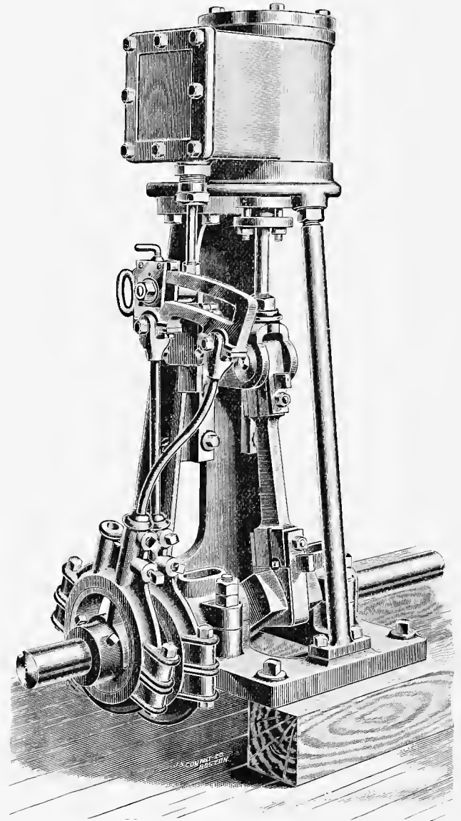
THE MORRIS SINGLE MARINE ENGINE.
